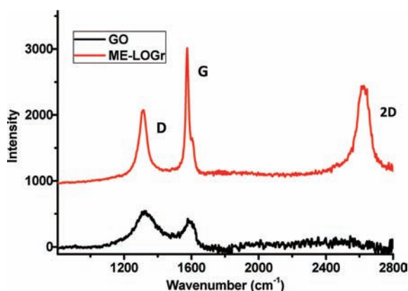
Figure 2. Raman spectra of ME-LOGr (red) and GO (black). The small intensity ratio of D/G bands and the high intensity of the 2D band in ME-LOGr are in contrast to the larger D/G band ratio and the absence of a 2D band in GO, indicating ME-LOGr has more ideal graphitic structures without adsorbent-induced surface modification.
