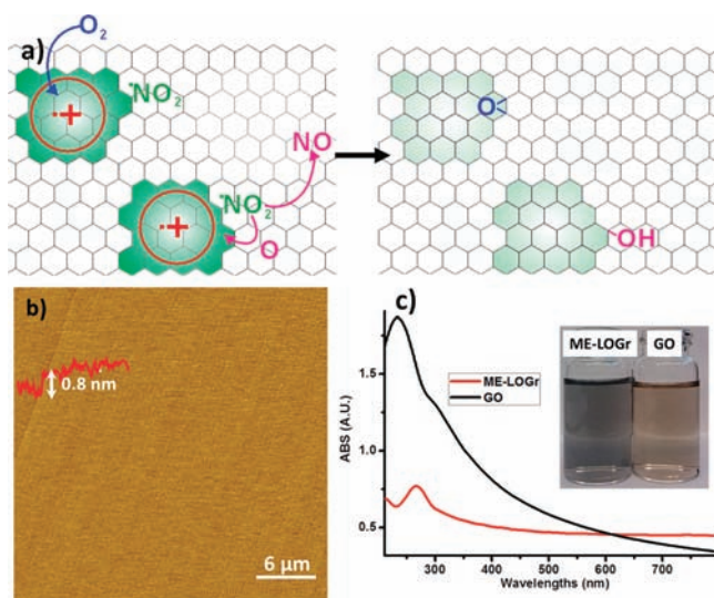
Figure 1. (a) Schematic drawing showing the proposed oxidation mechanism to directly produce highly conductive, low-oxygen-containing amphiphilic graphene sheets. A nitronium ion forms a single electron transfer (SET) intermediate with a graphene layer, which is intercepted by a rapid oxygen transfer from molecular oxygen, affording an epoxy group, or from \text{NO}_2^+ to form an OH group. (b) AFM image of a large ME-LOGr sheet deposited on a freshly cleaved mica surface. (c) UV-vis spectra of ME-LOGr (red) and GO (black). Inset: digital photograph showing the different colorations of ME-LOGr and GO solutions in water.
