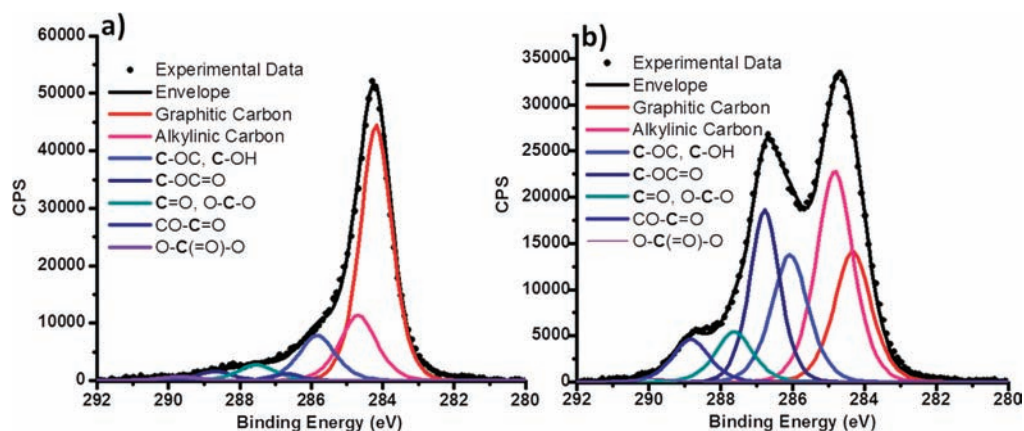
Figure 4. Carbon 1s core XPS spectra for thin films of (a) ME-LOGr and (b) GO. The content of oxygen-free carbon of ME-LOGr was 79%, which was comparable with the reported value of fully reduced GO, while GO (b) contains only 49% of oxygen-free carbon. This is direct evidence of much less oxidation in the ME-LOGr.
