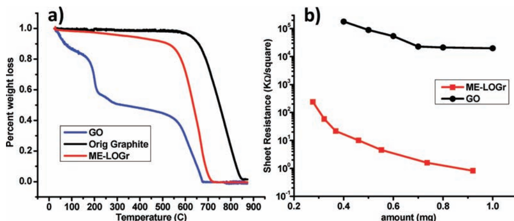
Figure 5. (a) TGA curves of % weight loss plotted against temperature, showing that ME-LOGr (red) is thermally much more stable than GO (blue) and highly comparable with its parent graphite (black). (b) Percolation study of ME-LOGr and GO using a four-point probe setup. After percolation threshold, the sheet resistivity of ME-LOGr (red) is 5 orders of magnitude lower than that of the heavily oxidized GO films.
