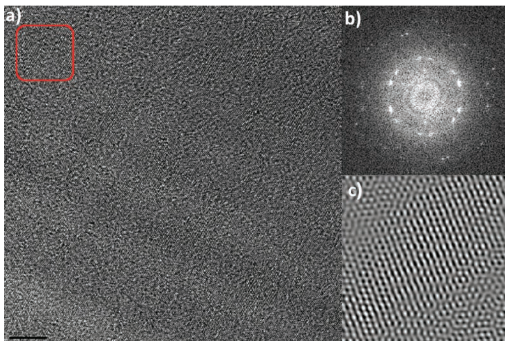
Figure 3. (a) Representative HRTEM image of ME-LOGr, which is composed of many different crystalline-like domains with average lateral size of 6–10 nm. No nanometer-sized holes were observed, which is highly in contrast to GO and rGO. The size of the crystalline domains is also much larger than those observed in GO and rGO. (b) Fast Fourier transform (FFT) pattern of the selected region indicated in (a). (c) The reconstructed image of the same spot as (b) after filtering with the frequency domain to include contributions from both sets of hexagons of the FFT pattern. The scale bar in (a) is 5 nm.
